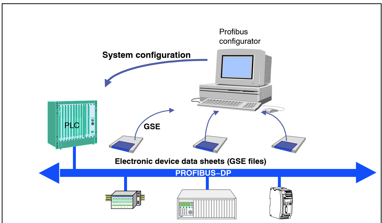
Fig. 2.1: Configuration with the aid of GSE files
