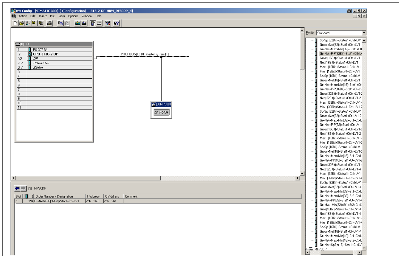
Fig. 2.8 : Configuration hardware
