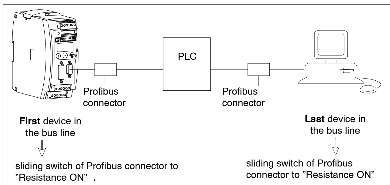
Fig. 3.1: Profibus operation
